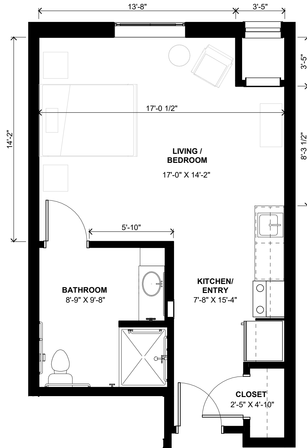
1 UNIT AL1 - FLOOR PLAN 1/4" = 1'-0" 0 3' 6'
