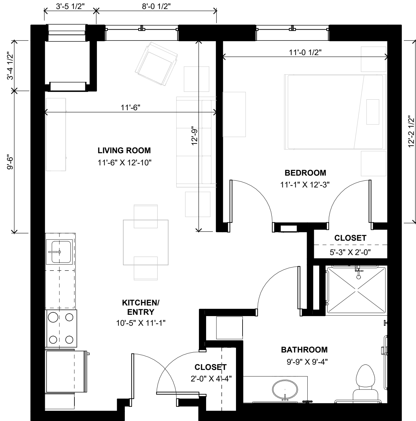
1 UNIT AL3 - FLOOR PLAN 1/4" = 1'-0" 0 3' 6'
