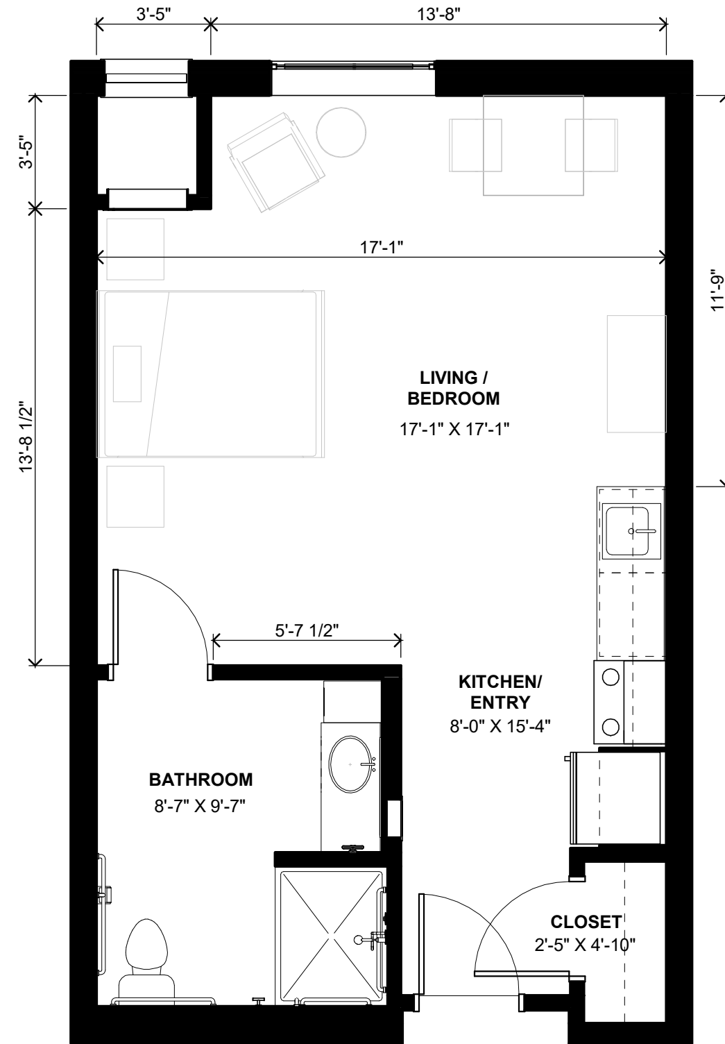
1 UNIT AL2 - FLOOR PLAN 1/4" = 1'-0" 0 3' 6'
