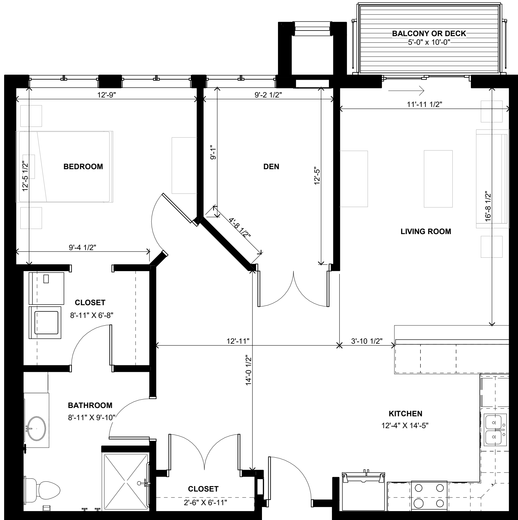
1 UNIT B1 - FLOOR PLAN 1/4" = 1'-0"
