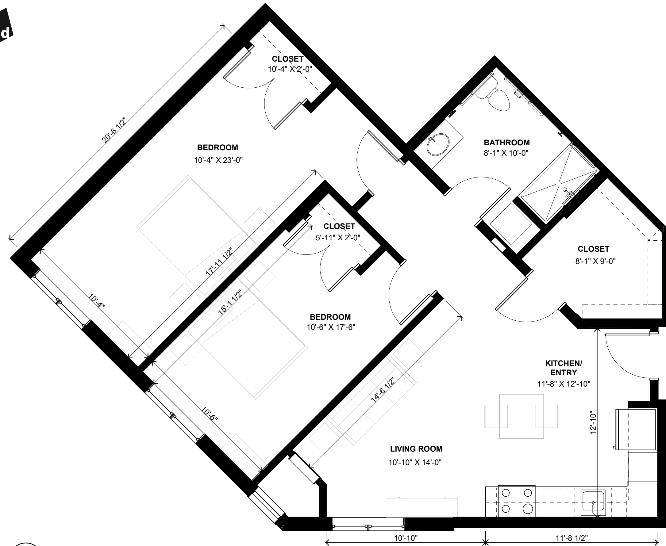
1 UNIT AL5 - FLOOR PLAN 1/4" = 1'-0" 0 3' 6'
